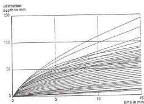
Figure 2.7 Accumulated infiltration versus time measured with 63 infiltrometers set at 1 m spacing on a 7 by 9 m grid in a sandy loam soil (Jaynes et al. 1988)
