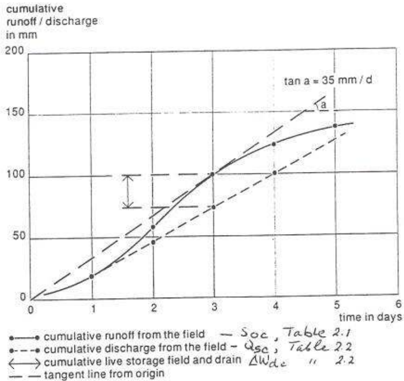
Figure 2.8 Runoff and discharge in time in example 2.7.
